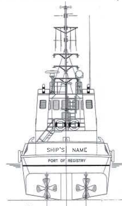
REAR VIEW
