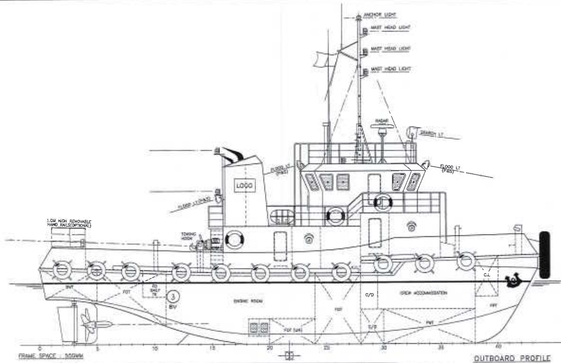
OUTBOARD PROFILE
