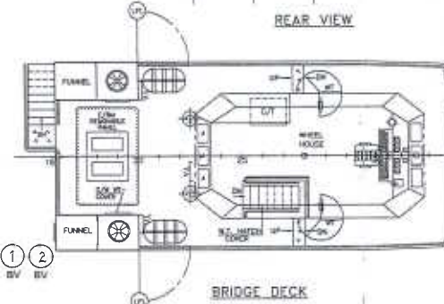
BRIDGE DECK
