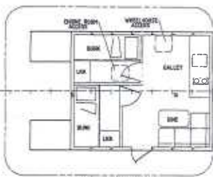
MAIN DECK PLAN
