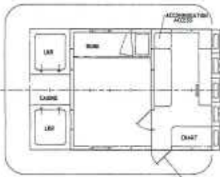
WHEELHOUSE PLAN
